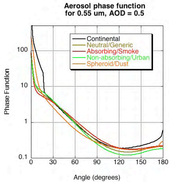
Figure 12: Plot of phase function at 0.55 \mu m (as a function of angle) for the 5 aerosol models in the V5.2 LUT. In each case, \tau = 0.5 .
