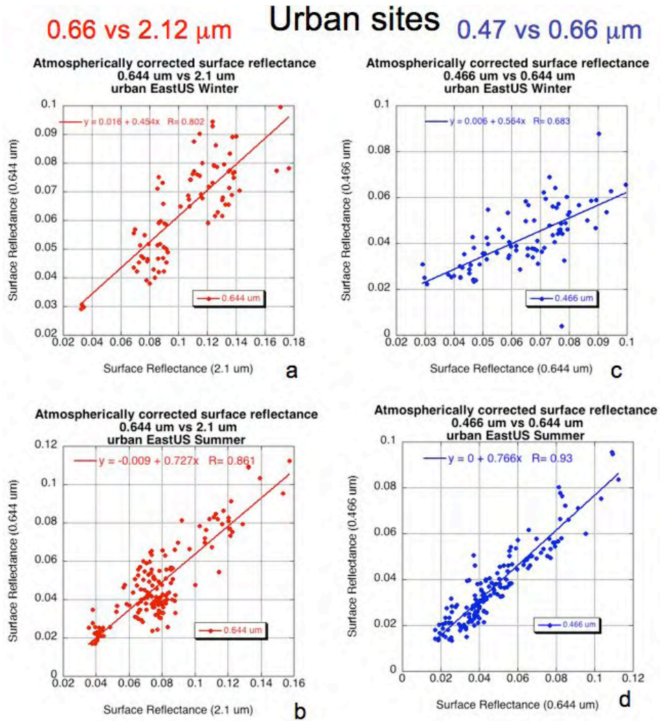
Figure 18: Surface Reflectance relationships for urban sites along the US East Coast. The left two subfigures (a-b) are for 0.66 \mu\text{m} versus 2.12 \mu\text{m} channels, whereas the right two subfigures (c-d) are for 0.47 \mu\text{m} versus 0.66 \mu\text{m} channels. From the top to bottom, subfigures (a) and (c) are for the sites in winter, and (b) and (d) are for the sites during summer.
