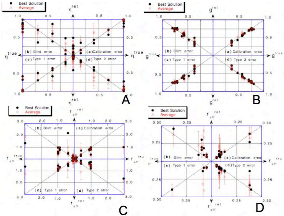
Figure 7: Same as Fig 6 but for (A) ratio \eta , (B) asymmetry parameter g , (C) Effective Radius ( R_{eff} ) and for (D) blowup of Effective Radius ( R_{eff} ) < 0.40 . Error bars correspond to the standard deviation of the 'average' solution.
