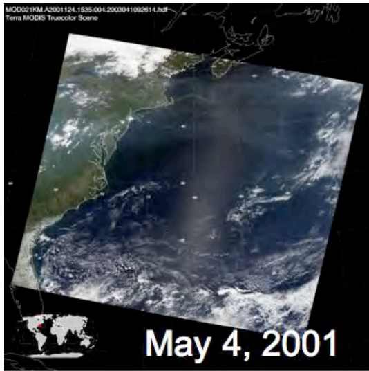
A) RGB: \rho^M(0.66,0.55,0.47 \mu\text{m})
