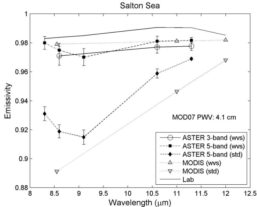
Figure 16. Emissivity spectra comparisons on June 15, 2000 over the Salton Sea between ASTER (3-band), ASTER (5-band), and MODTES, using the TES algorithm along with lab spectra of water from the ASTER spectral library. Results from the WVS method and the STD atmospheric correction are also shown. An estimate of the PWV from the MOD07 atmospheric product indicates very high humidity on this day.
