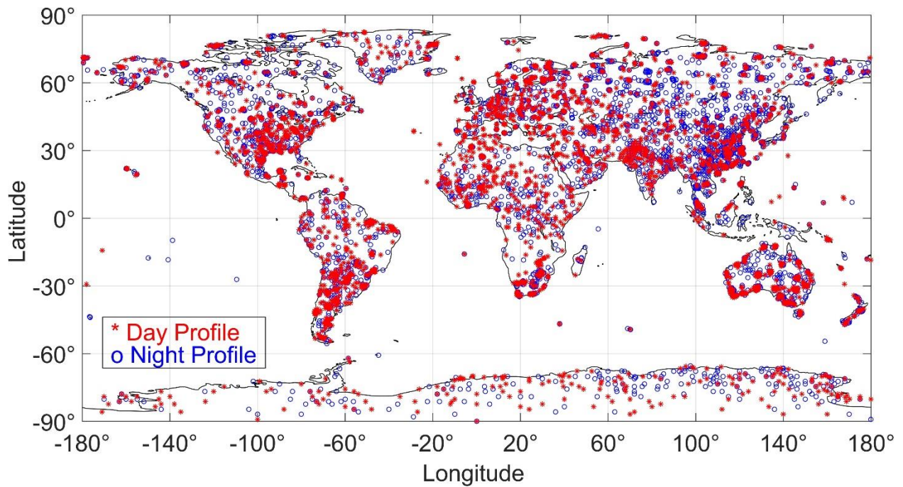
Figure 7. Global SeeBor radiosonde database showing the distribution of day (red stars) and night (open blue circles) profiles used in the generation of the WVS coefficients.
