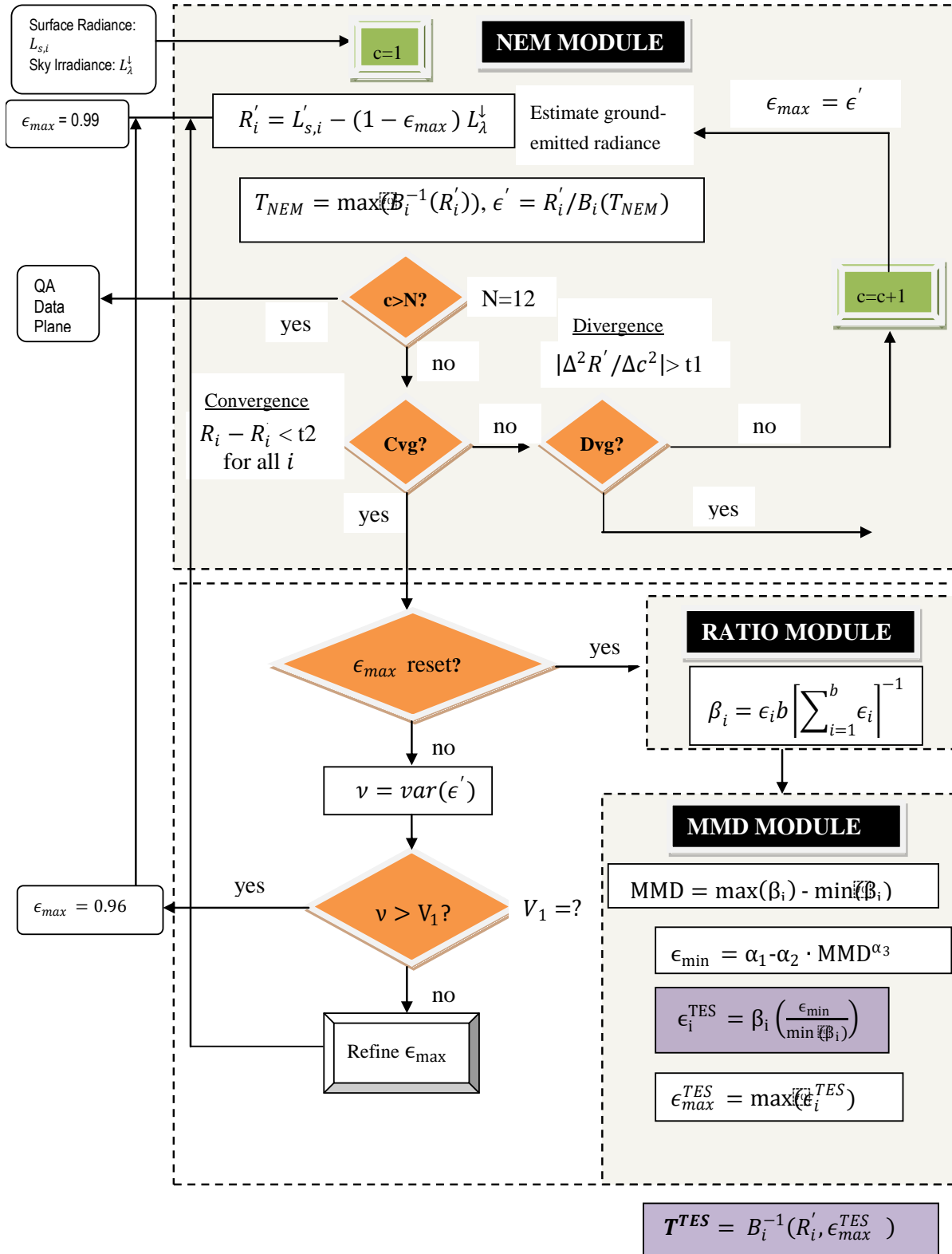
Figure 12. Flow diagram of the TES algorithm in its entirety, including the NEM, RATIO, and MMD modules.
