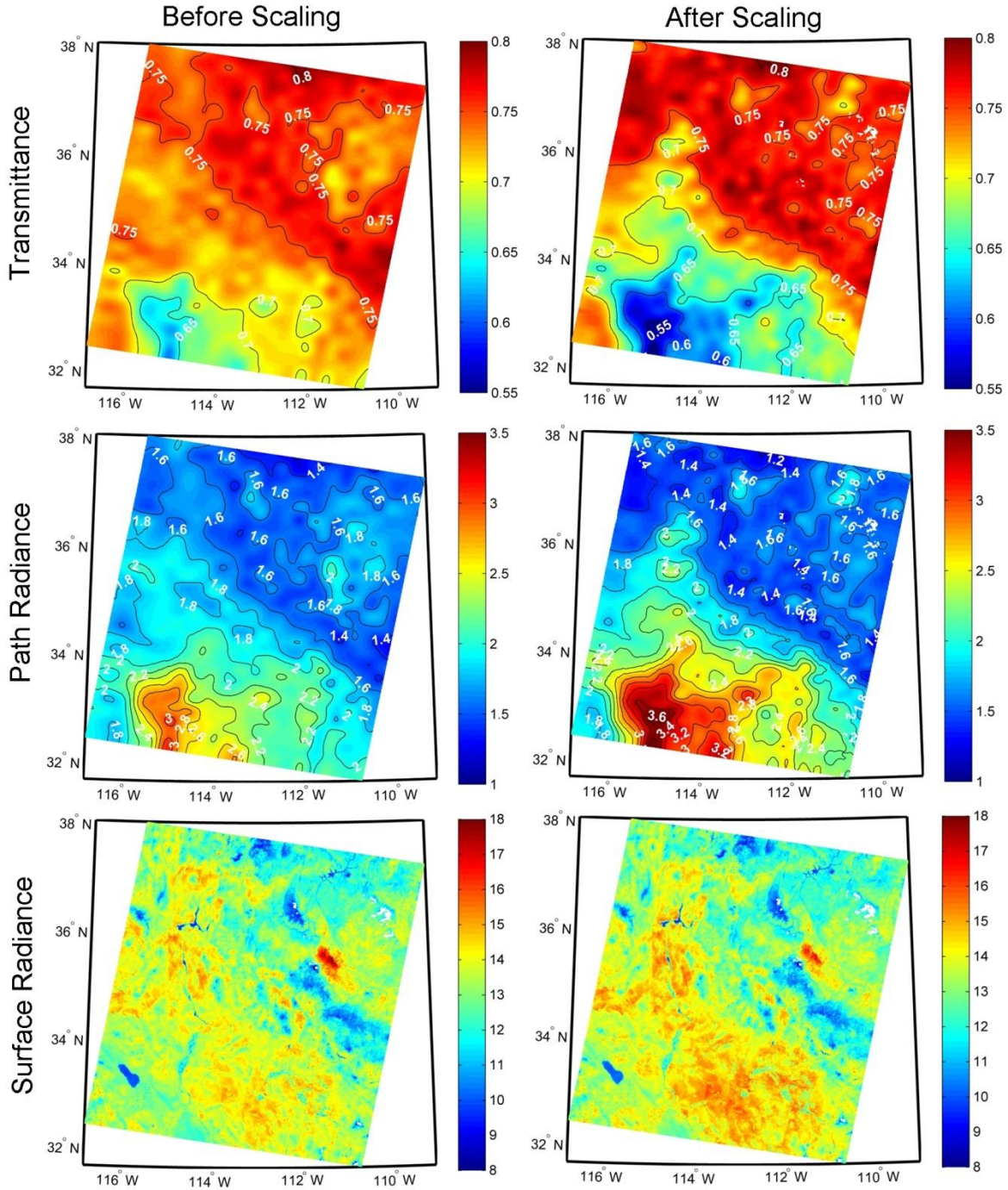
Figure 5. Comparisons between the atmospheric transmittance (top), path radiance ( W/m^2/\mu m^{-1} ) (middle), and computed surface radiance ( W/m^2/\mu m^{-1} ) (bottom), before and after applying the WVS scaling factor \gamma to a MODIS scene cutout shown in Figure 5. Results are shown for MODIS band 29 ( 8.55 \mu m ).
