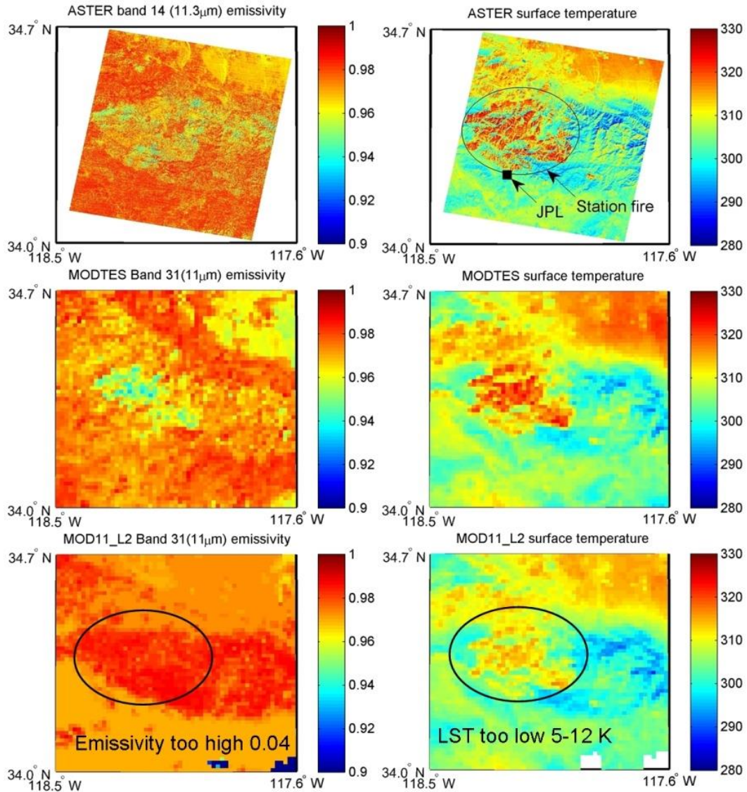
Figure 17. Emissivity images (left) and surface temperature images (right) for ASTER (top), MODIS TES (MODTES) (center) and MODIS SW (MOD11_L2) (bottom) products over the Station Fire burn scar just north of Pasadena, CA. Location of JPL in Pasadena and burn scar area indicated at top right. MODTES and ASTER results match closely; however, the MOD11_L2 temperatures are underestimated by as much as 12 K, due to an incorrect emissivity classification.
