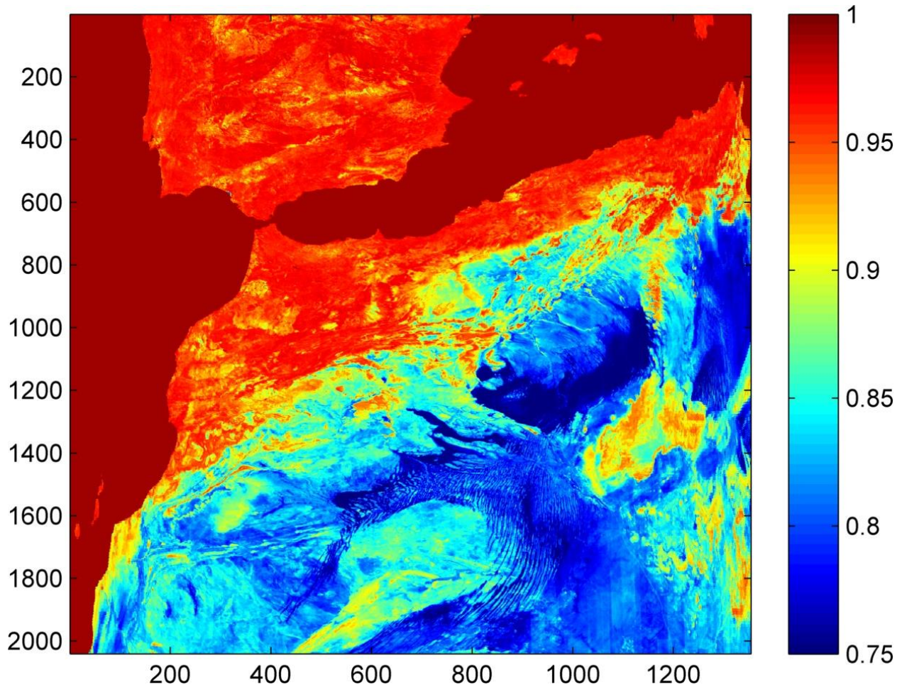
Figure 9. Spectrally adjusted ASTER GED emissivity for MODIS band 29 (see text for details). The ASTER GED emissivity (100 m) has been geolocated onto the MODIS swath (1-km) and has been adjusted for vegetation phenology using the MODIS MOD13 NDVI product.
