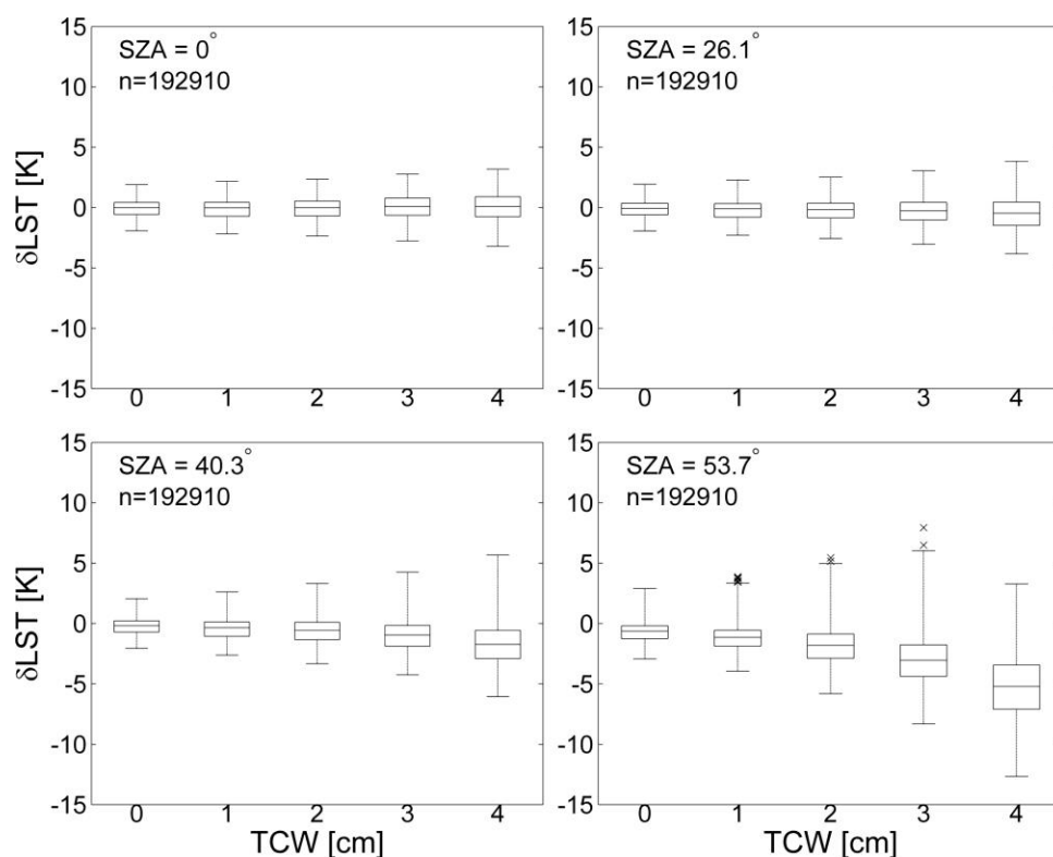
Figure 20. MODIS LST uncertainties using the TES algorithm versus TCW for four viewing Gaussian angles of 0^\circ , 26.1^\circ , 40.3^\circ , and 53.7^\circ . The value n represents the number of data points used for a specific land surface type, in this case bare surfaces (rocks, soils, sands).
