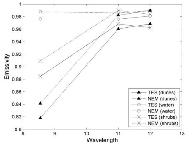
Figure 14. MODIS derived TES and NEM emissivity spectra for three different surface types for the MODIS cutout shown in Figure 11: Algodones Dunes, Salton Sea, and shrublands (mixed soil and vegetation). Details of the TES and NEM outputs from these spectra are shown in Table 7.
