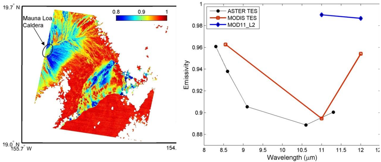
Figure 18. (left) ASTER band 12 (9.1 \mu\text{m} ) emissivity image over Mauna Loa caldera, Hawaii on 5 June 2000, and (right) emissivity spectra from ASTER, MODTES, and MOD11 emissivity classification. While ASTER and MODTES agree closely, MOD11 emissivities are too high, resulting in large LST discrepancies between MODTES and MOD11 (12 K) due to misclassification in bands 31 (11 \mu\text{m} ) and 32 (12 \mu\text{m} ).
