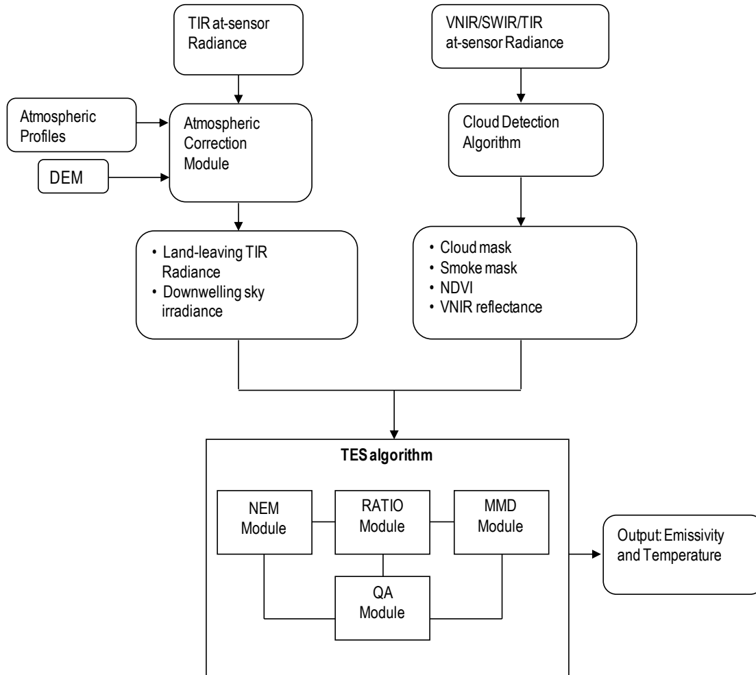
Figure 11. Flow diagram showing all steps in the retrieval process in generating the MODIS MOD21 LST&E product starting with TIR at-sensor radiances and progressing through atmospheric correction, cloud detection, and the TES algorithm.
