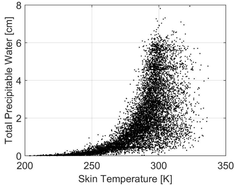
Figure 6. The total precipitable water versus skin temperature in the SeeBor profile used in the simulation for generating view angle and day–night-dependent coefficients.
