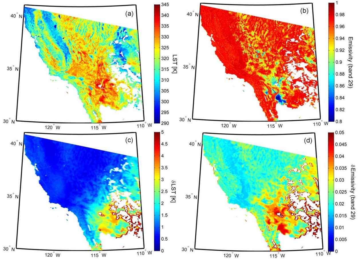
Figure 21. MODIS TES retrievals including WVS correction over the southwestern United States on 7 August 2004: (a) (top left) LST, (b) (top right) emissivity for band 29 (8.55 μm), (c) (bottom left) LST uncertainty, and (d) (bottom right) emissivity uncertainty for band 29 (8.55 μm). White areas over land indicate areas of cloud that have been masked out using the MOD35 cloud mask product.
