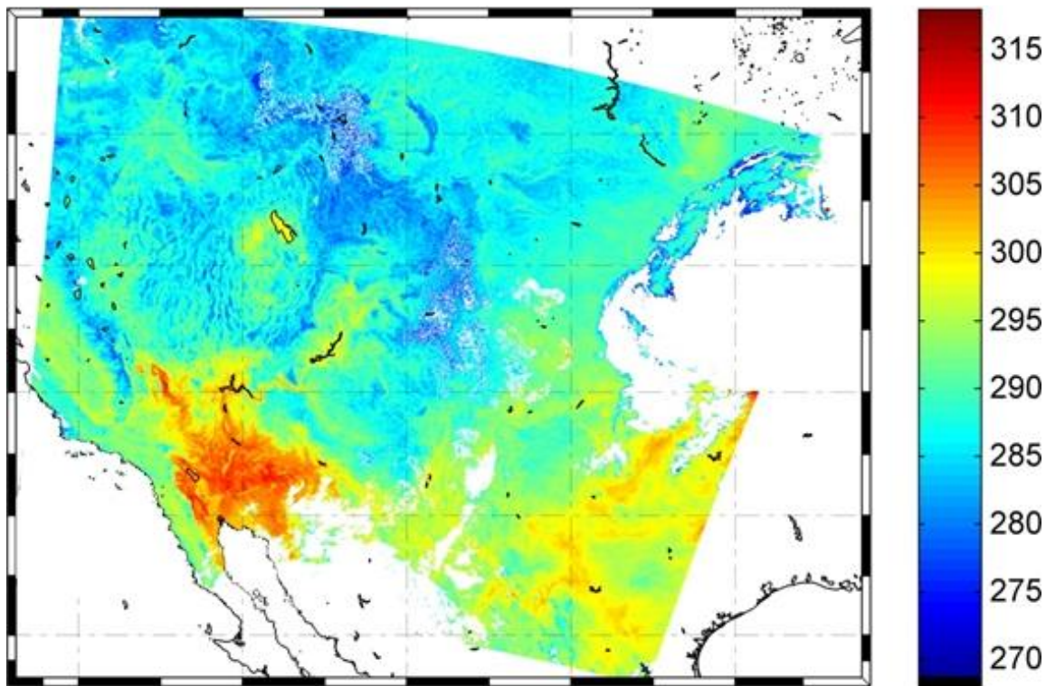
Figure 1. Example MxD21_L2 LST granule (2006195) over southwestern USA (degrees K).
