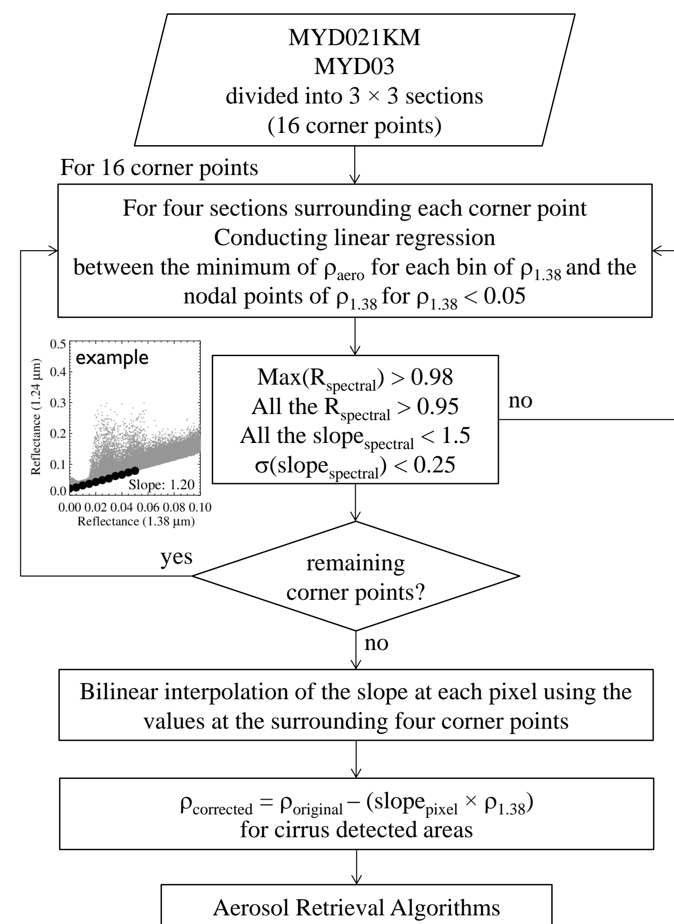
Figure 1. Flowchart of the TOA reflectance correction for thin cirrus signals.
