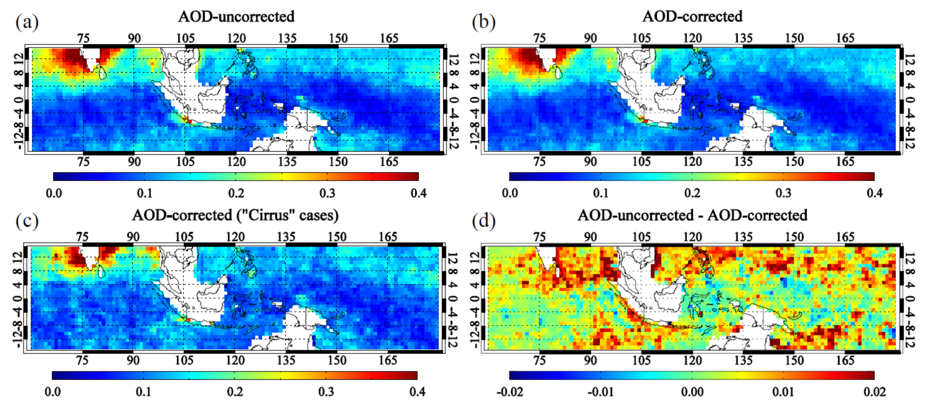
Figure 6. Spatial distribution of seasonal mean AOD for (a) AOD-uncorrected, (b) AOD-corrected, (c) AOD-corrected for cirrus-present cases, and (d) seasonal mean AOD difference over the eastern tropics for the period from 1 March 2007 to 31 May 2007.
