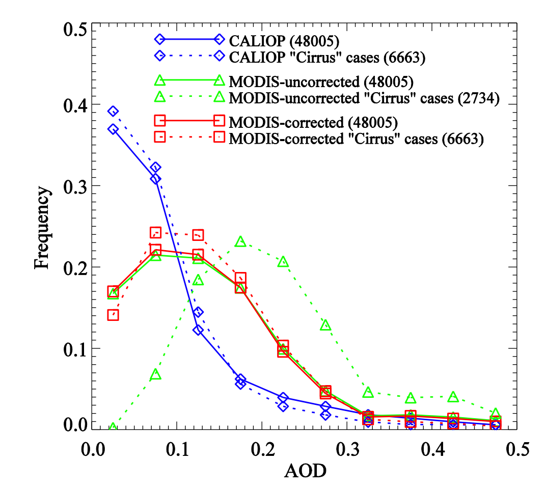
Figure 5. Normalized frequency distribution of CALIOP AOD and MODIS AOD data sets for different conditions. The same data coverage and period as used in Figure 4.
