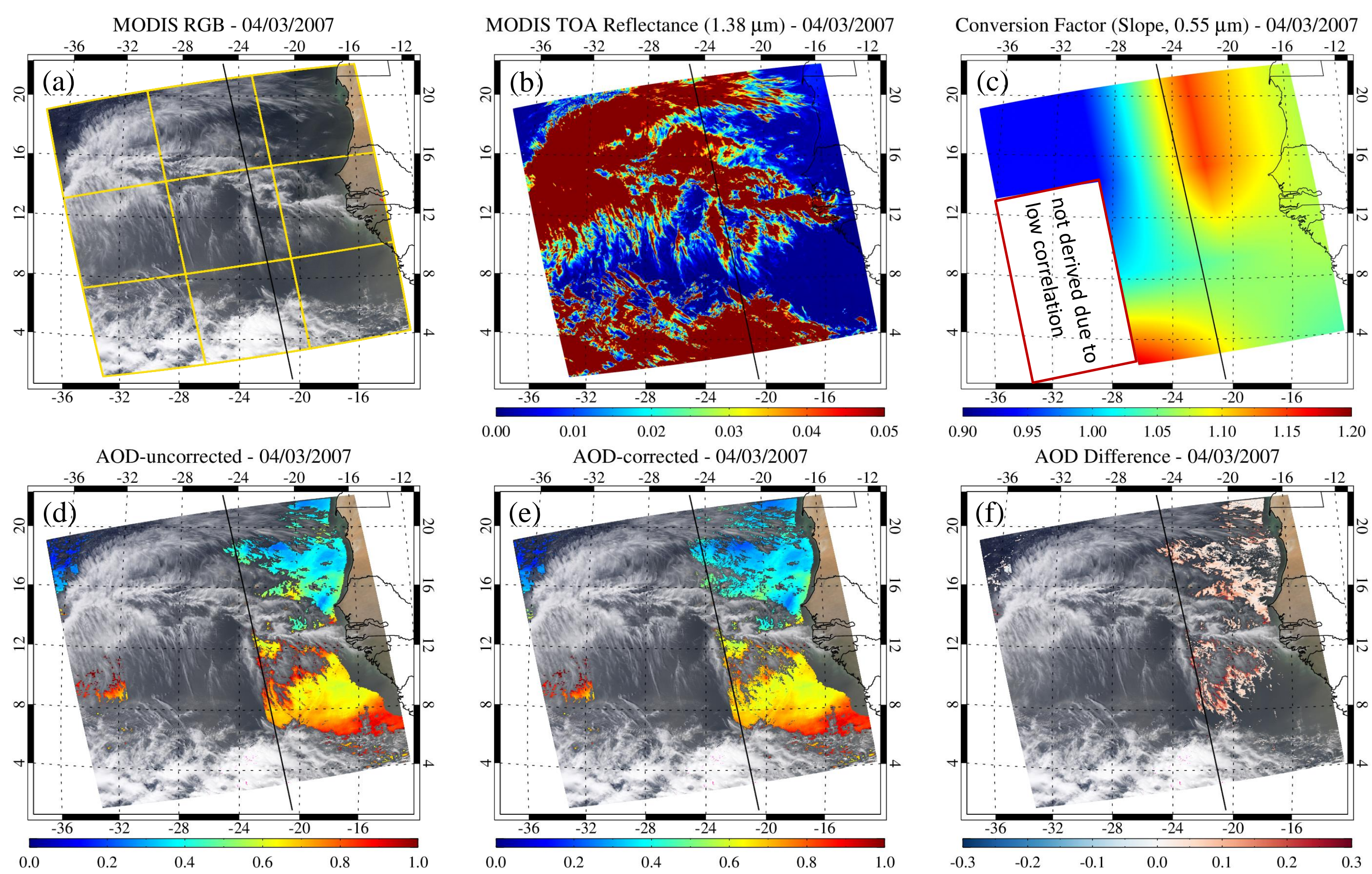
Figure 2. (a) MODIS RGB image, (b) TOA reflectance at 1.38 \mu\text{m} , (c) \rho_{1.38} -to-aerosol band conversion factors at 0.55 \mu\text{m} , (d) AOD without cirrus correction, (e) AOD with cirrus correction, and (f) AOD correction magnitude (AOD-uncorrected - AOD-corrected). Data for the MODIS granule collected at 15:05 UTC on 4 March 2007. The black line represents the CALIOP observation track.
