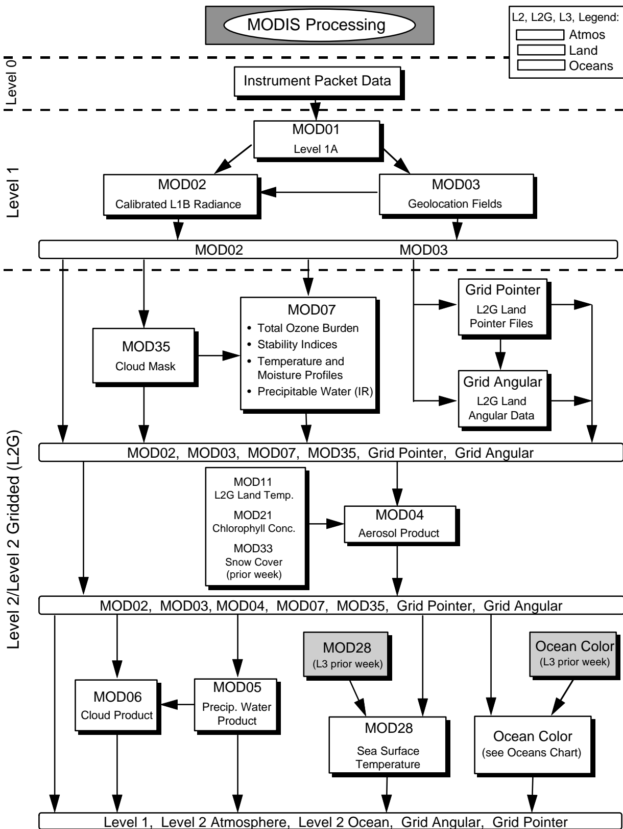
Flow Diagram Showing Interrelationship of MODIS Atmosphere, Land, and Ocean Products.
